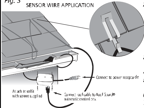
Fig. 3 SENSOR WIRE APPLICATION
